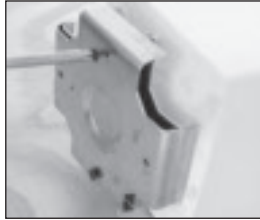
2. Remove fastening plates from bottom of post. Trim top of post leaving the pipe flush with the outer shell.
